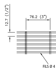
DETAILS MAILLE
